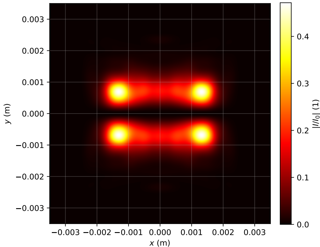
Intensity profile I(x, y, z = 2.946)/I_0 , P_{in}=4.0P_{cr} , artificial time
